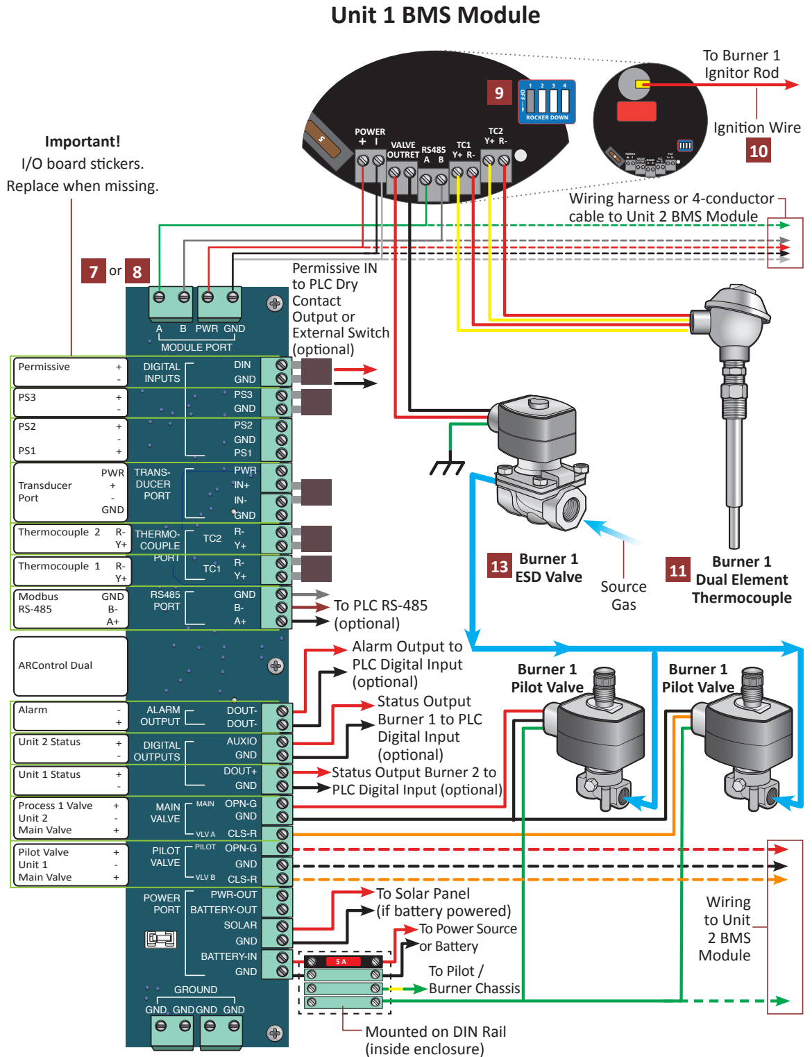
Image 1.1.1 • Unit 1 & Unit 2 BMS Module wiring diagram
